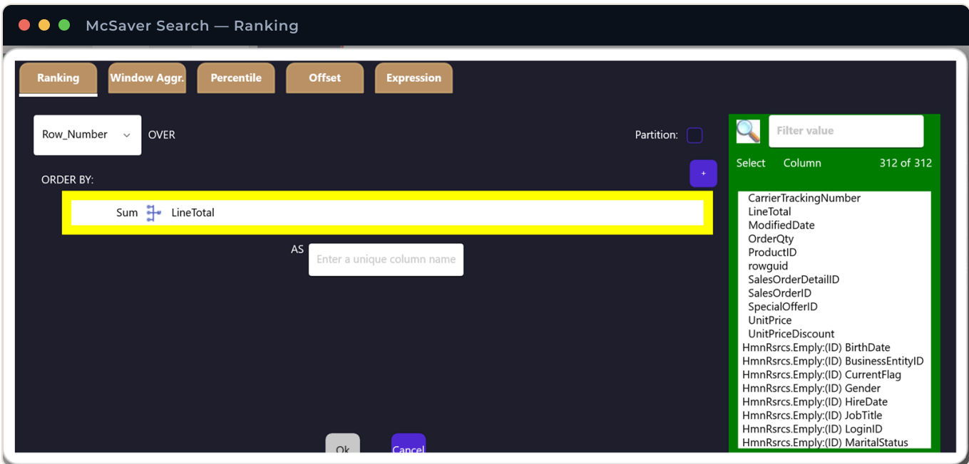
The Ranking tab of the Select column editor — a ROW_NUMBER window function with OVER and an ORDER BY.
